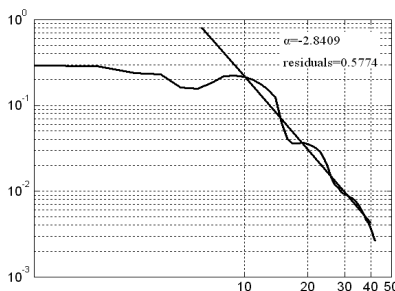
Figure 5: PSD revealed a 1/f^\alpha form with upward deviations on the beta and gamma range, \alpha varied from -1 to -3.
