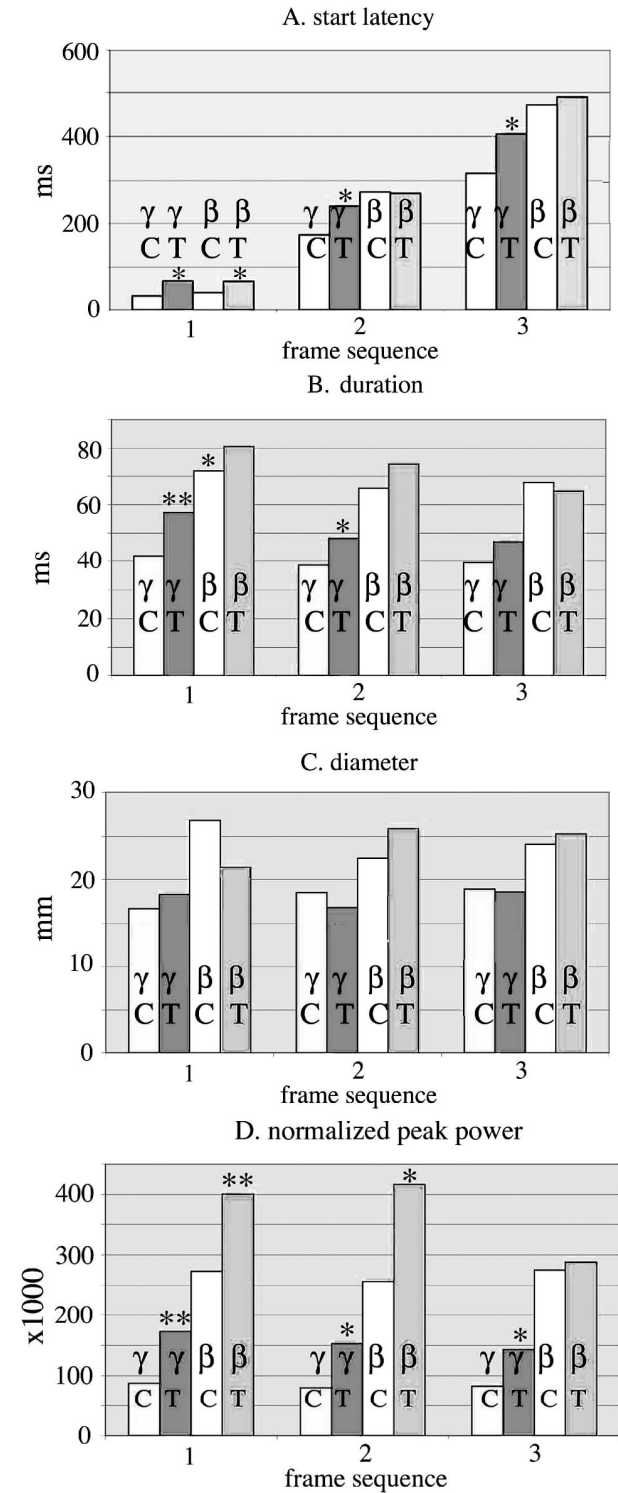
Fig. 6. Summary of wave packet parameters. From Freeman (2005).
