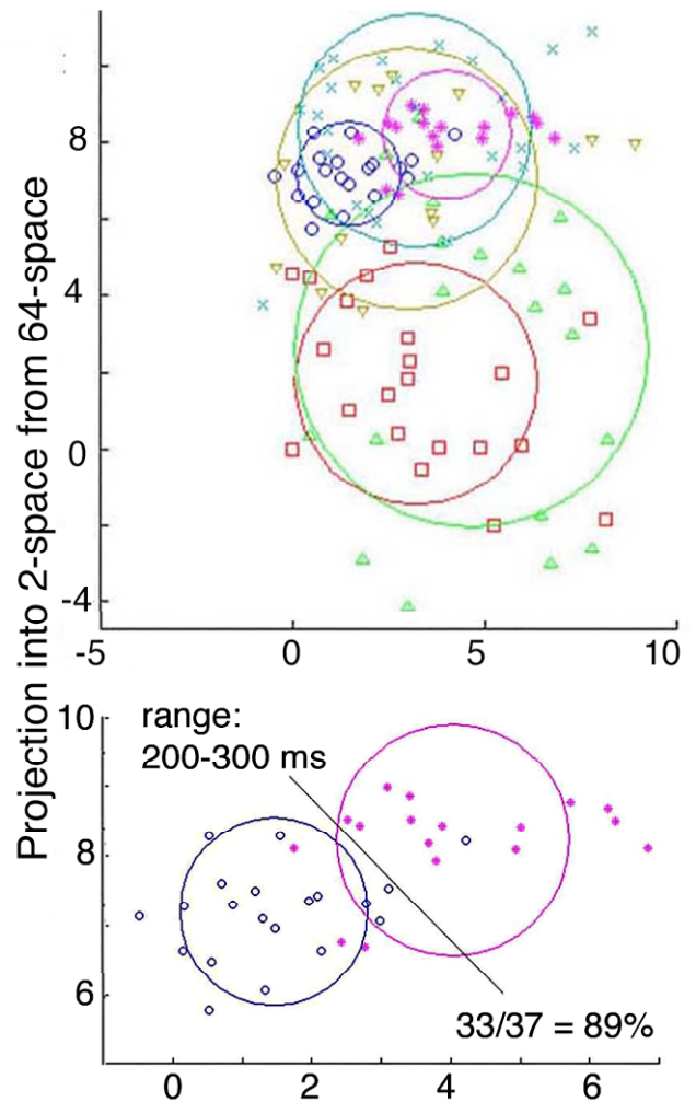
Fig. 5. Feature vectors from 40 trials are represented by points after projection from 64-space into 2-space by nonlinear mapping.
