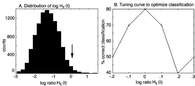
Fig 3. Use of tuning curves to locate classifiable EEG segments..
