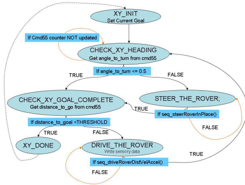
Figure 3. Finite State Machine cruise_XY_Z used for the SODAS navigation control
