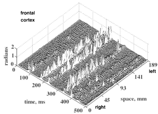
FIG. 8. The temporal numerical differences approximated the time derivative of the analytic phase on lines parallel to the left abscissa at 5 ms intervals. The data were the 64 EEGs from the curvilinear array placed over the frontal lobes across the midline. The channels were spaced at 3 mm intervals as shown on the right abscissa. The plateaus indicated stability of phase. The spikes were the jumps in rate of change in phase. For display the absolute values of the differences were weighted by Eq. (2). The temporal pass band was optimized at 12–30 Hz by maximizing the cross correlation of the signed derivative with the raw EEG in the alpha range of the spectrum. Spatial synchrony was indicated by alignment of the jumps in phase parallel to the right abscissa. A traveling wave would have appeared along a diagonal line. This parallel alignment was independent of the orientation of the array on the scalp.
