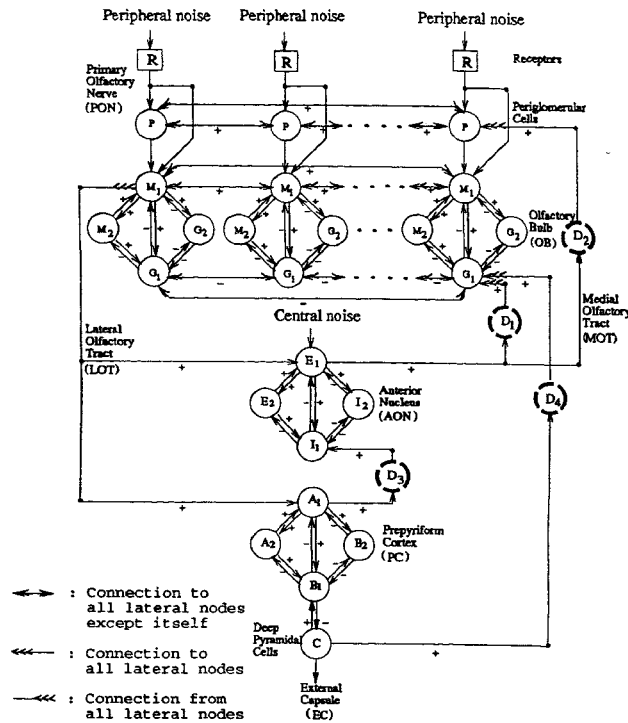
Figure 6. A flow diagram is constructed from anatomical connection data and used to specify the inputs and outputs of a set of coupled ODEs. Each node, F_i , sums inputs from all other nodes, v_j , after the sigmoid conversion, G , and the synaptic weights, k_{ij} , i \neq j (no neuron acts synaptically onto itself):
